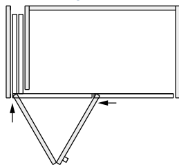
Hawa Folding Concepta III 25 Pull, links Aluminium, eloxiert
