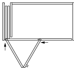
Hawa Folding Concepta III 20 Pull, links Aluminium, eloxiert
