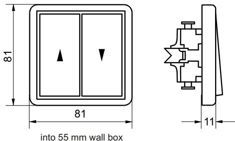
Flush mounting (529200)
