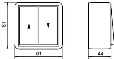
Surface mounting (529000)
