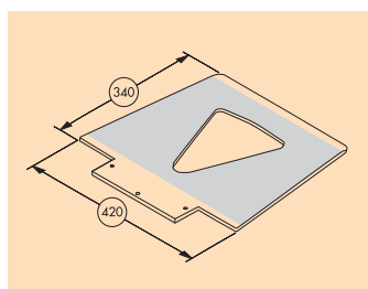
3 Art.-Nr. E/1543.930003 Schaufel G
