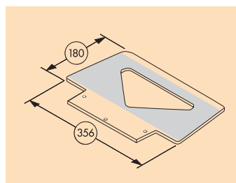
5 Art.-Nr. E/1543.930018 Schaufel WL
